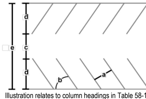
Figure 60-1: Illustration of Parking Standard Dimensions
