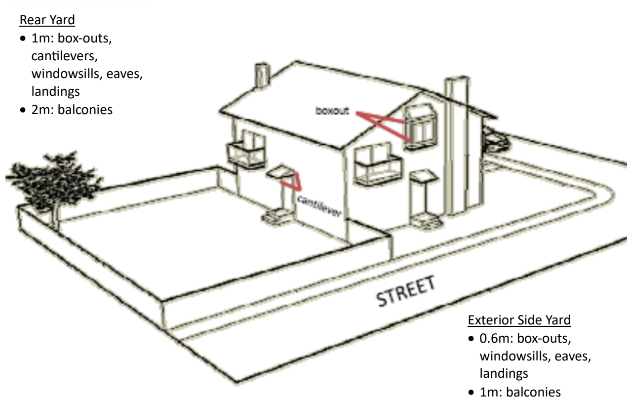
Figure 55-2: Permitted Projections – Rear and Exterior Side Yard Setbacks
